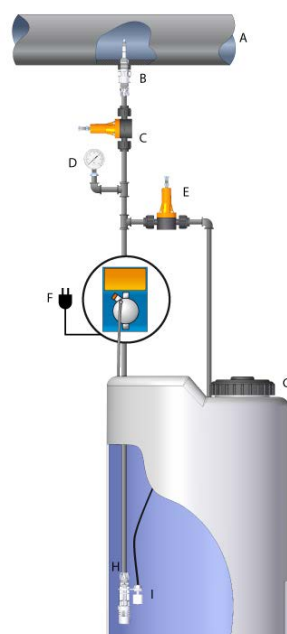
Fig. 6 - Installation type
